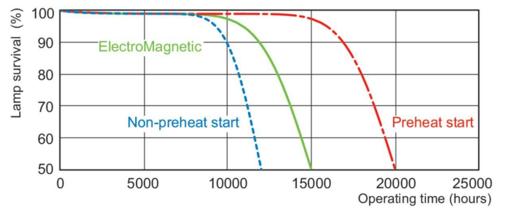
Life Expectancy Diagram - MASTER TL-D Food 58W/79 SLV/25
